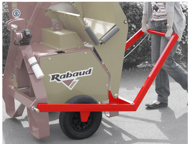
Transport trolley with 2 wheels (for XYLOSCIE 700 ET)
